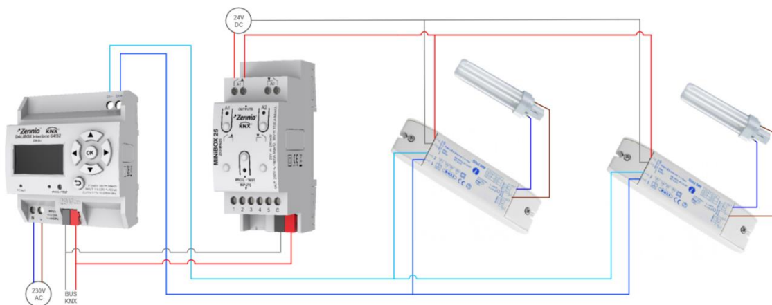
Figure 16. Wiring suggestion for the Standby function
