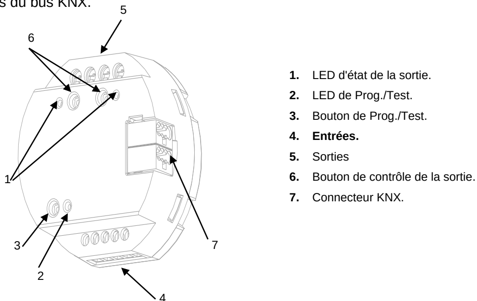
Figure 1. inBOX 24 vT. Éléments.
